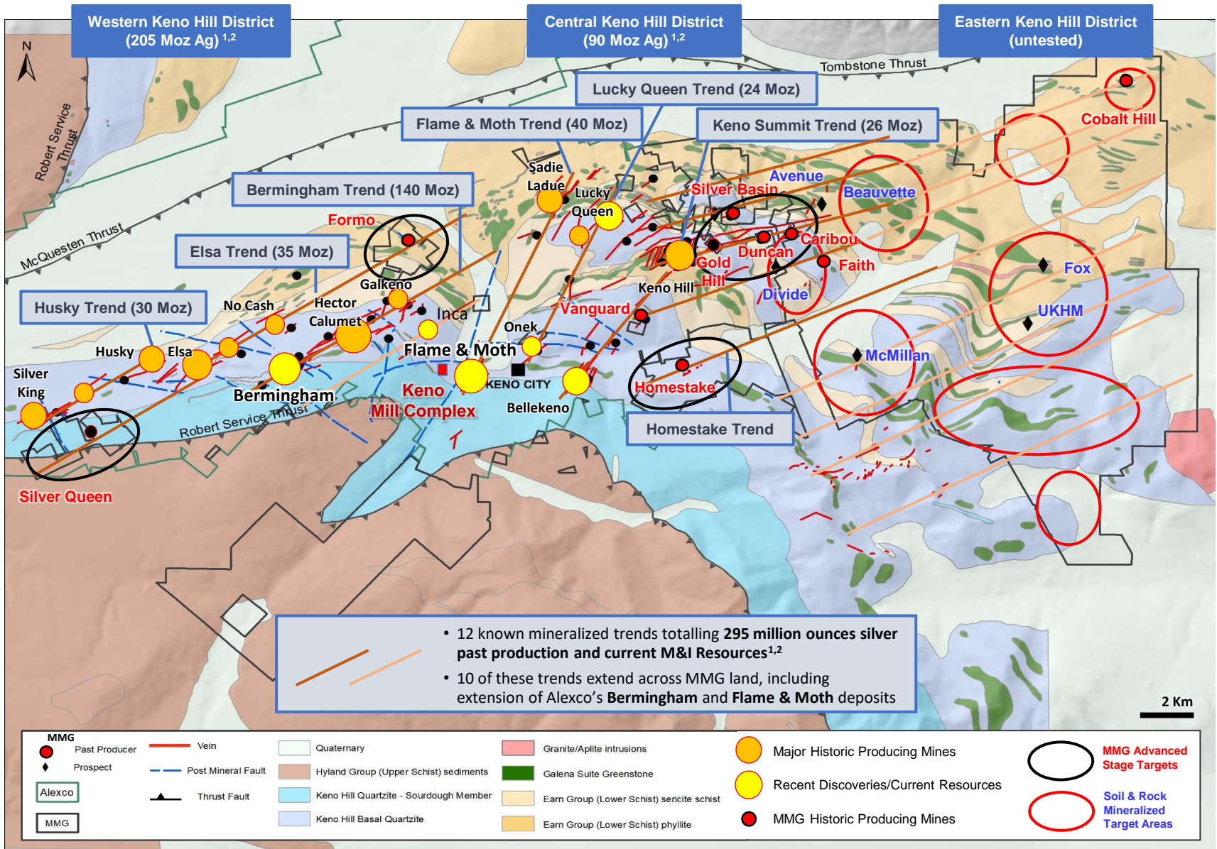
FIGURE 1 – KENO SILVER DISTRICT GEOLOGY AND DEPOSITS
