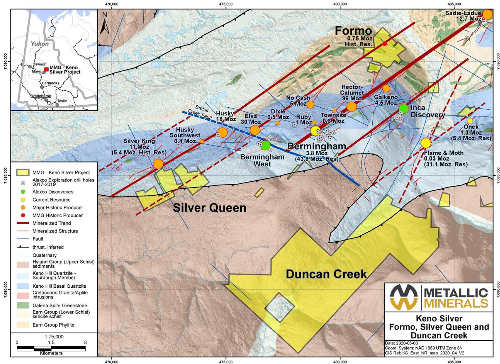
FIGURE 2 – WESTERN KENO SILVER DISTRICT WITH FORMO, SILVER QUEEN AND DUNCAN TARGET AREAS
